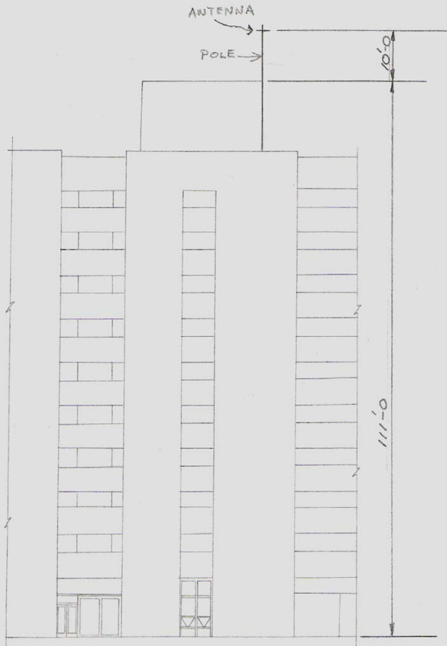
SOUTH ELEVATION
